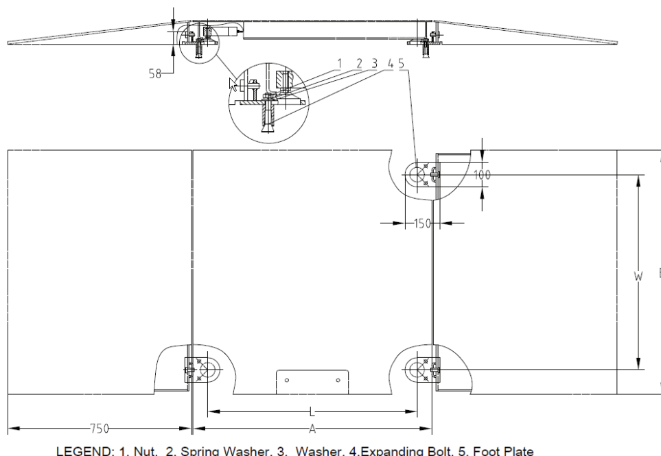
Figure 3. Optional Foot Plate and Ramp Installation
